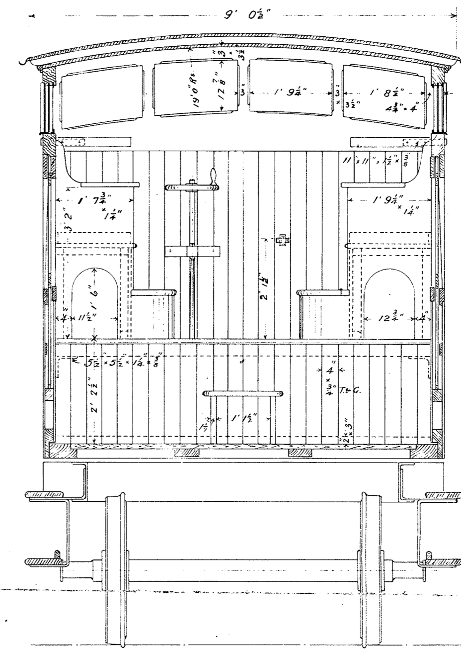
At B-B.
