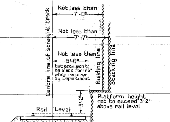
DIAGRAM SHOWING LATERAL CLEARANCES TO BE OBSERVED ON PRIVATE SIDINGS.
