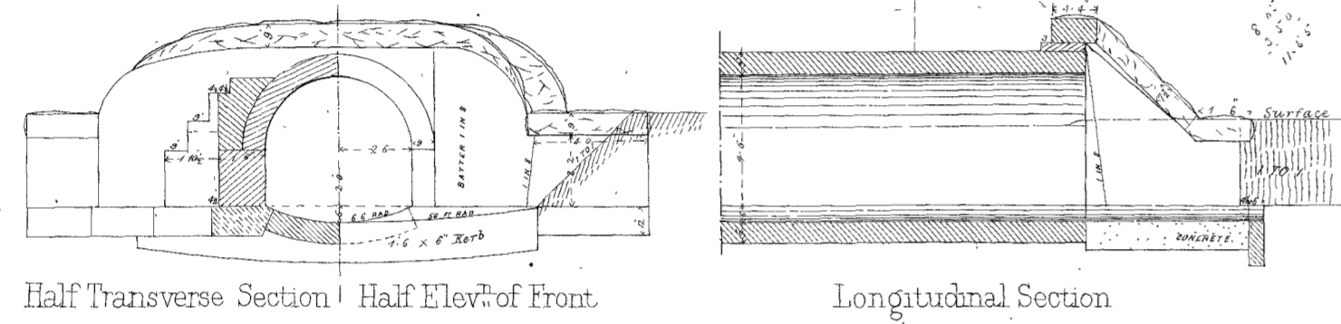
(Fig 1) 5' x 5' WITH CURVED WINGS
