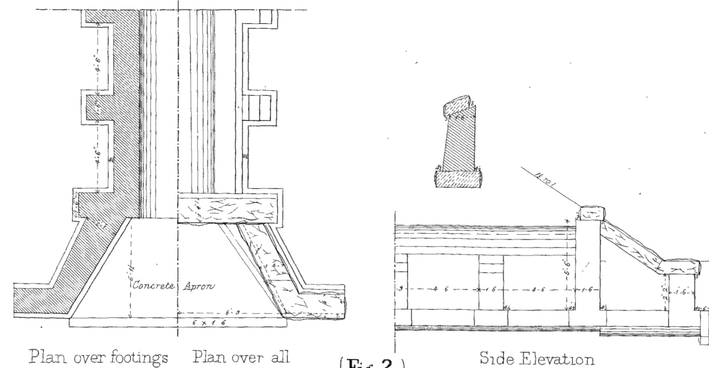
(Fig 2) 5' x 5' WITH STRAIGHT WINGS
