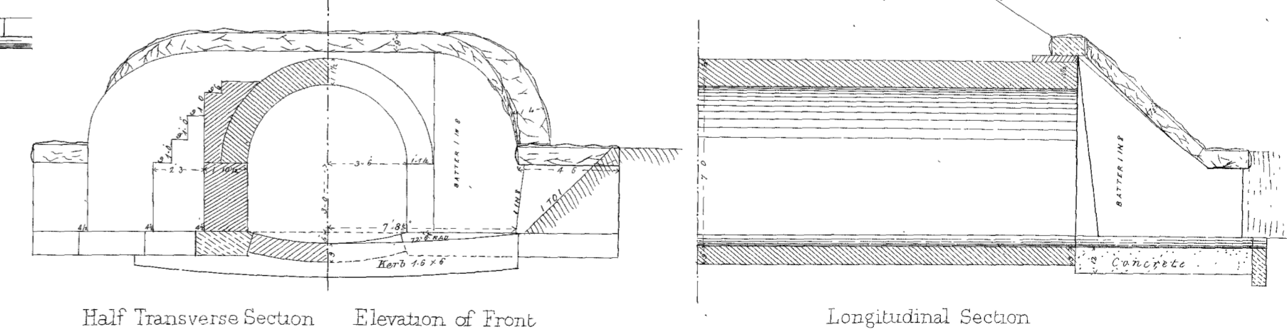
(Fig 6) 7' x 7' WITH CURVED WINGS
