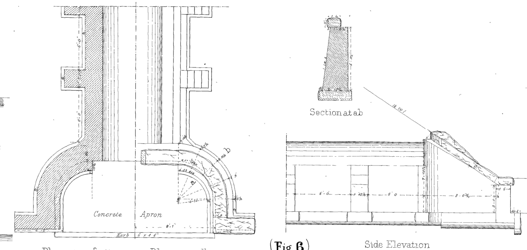
(Fig 6) 7' x 7' WITH CURVED WINGS
