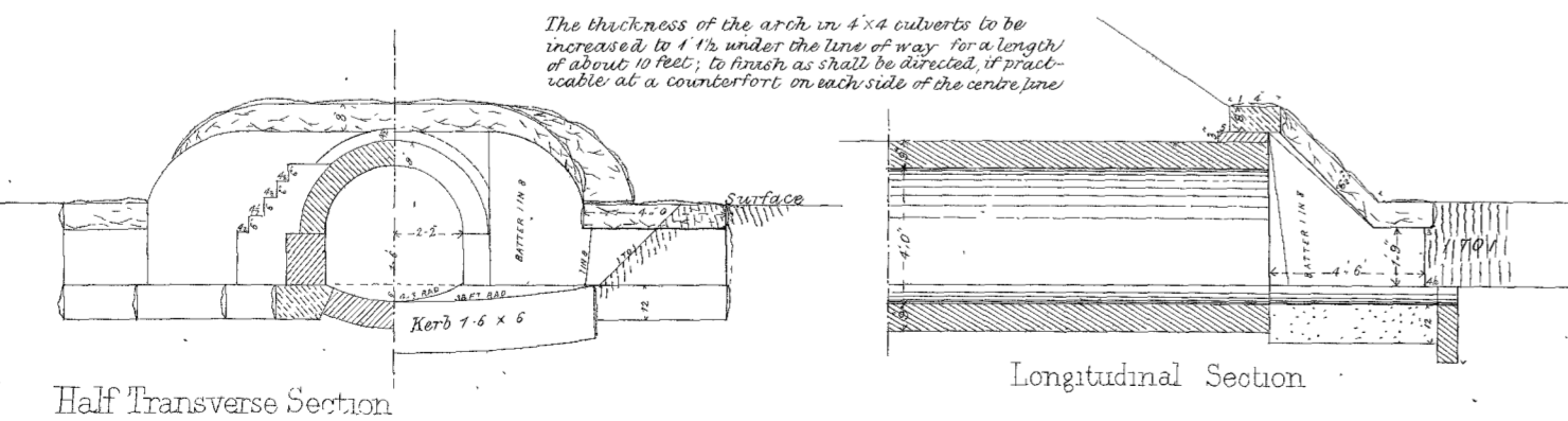
(Fig 3) 4' x 4' WITH CURVED WINGS
