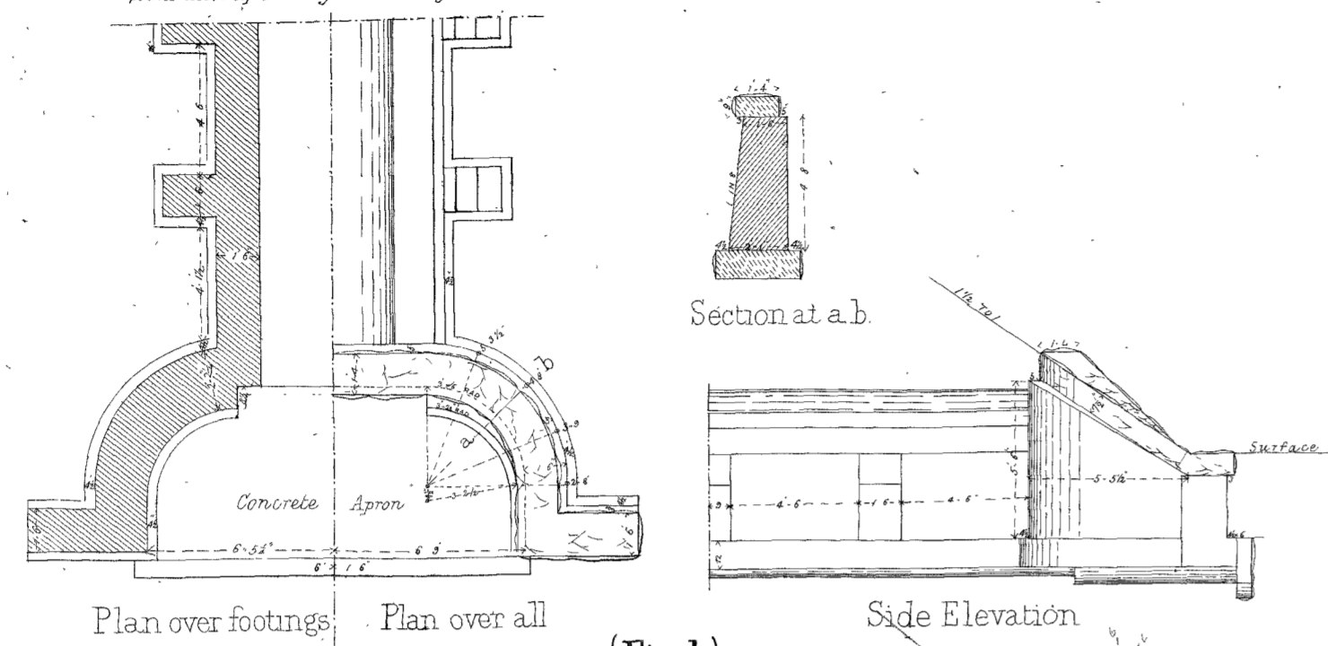
(Fig 1) 5' x 5' WITH CURVED WINGS
