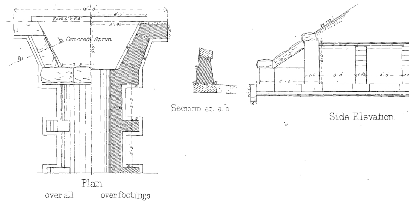
(Fig 4) 4' x 4' WITH STRAIGHT WINGS
