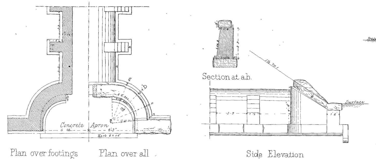
(Fig 3) 4' x 4' WITH CURVED WINGS
