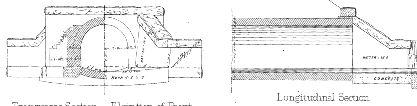
(Fig 2) 5' x 5' WITH STRAIGHT WINGS
