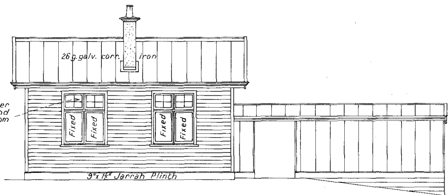
— ELEVATION TO APPROACH —
