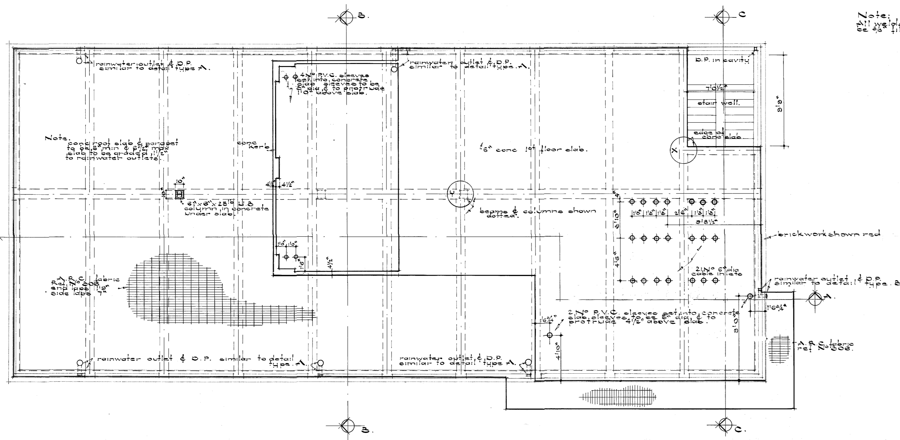
PLAN OF ROOF SLAB LEVEL FIRST FLOOR LEVEL scale: 1/4" = 1'-0"
