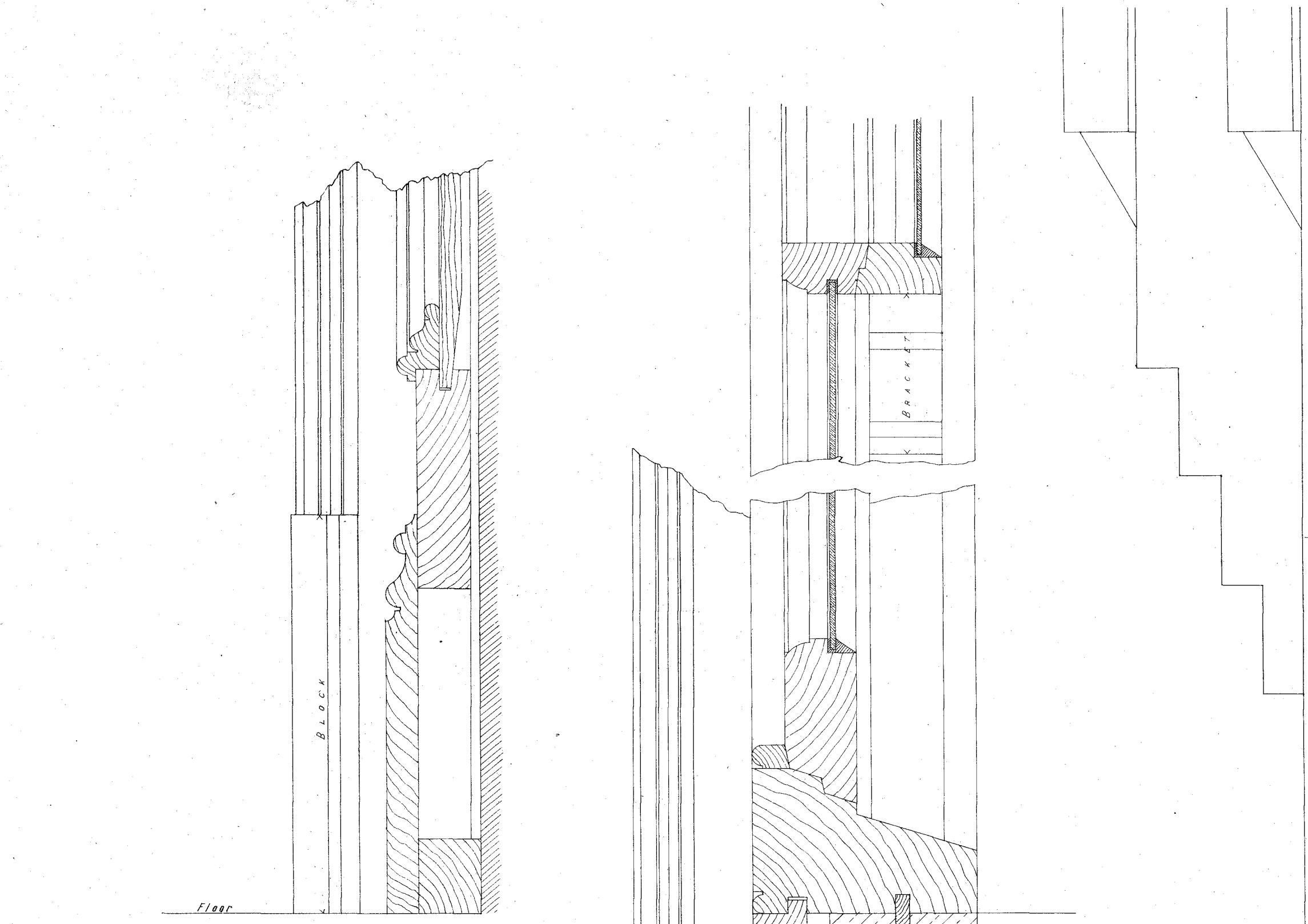
SECTION THROUGH BOTTOM RAIL & PLINTH OF WINDOW-BACK
