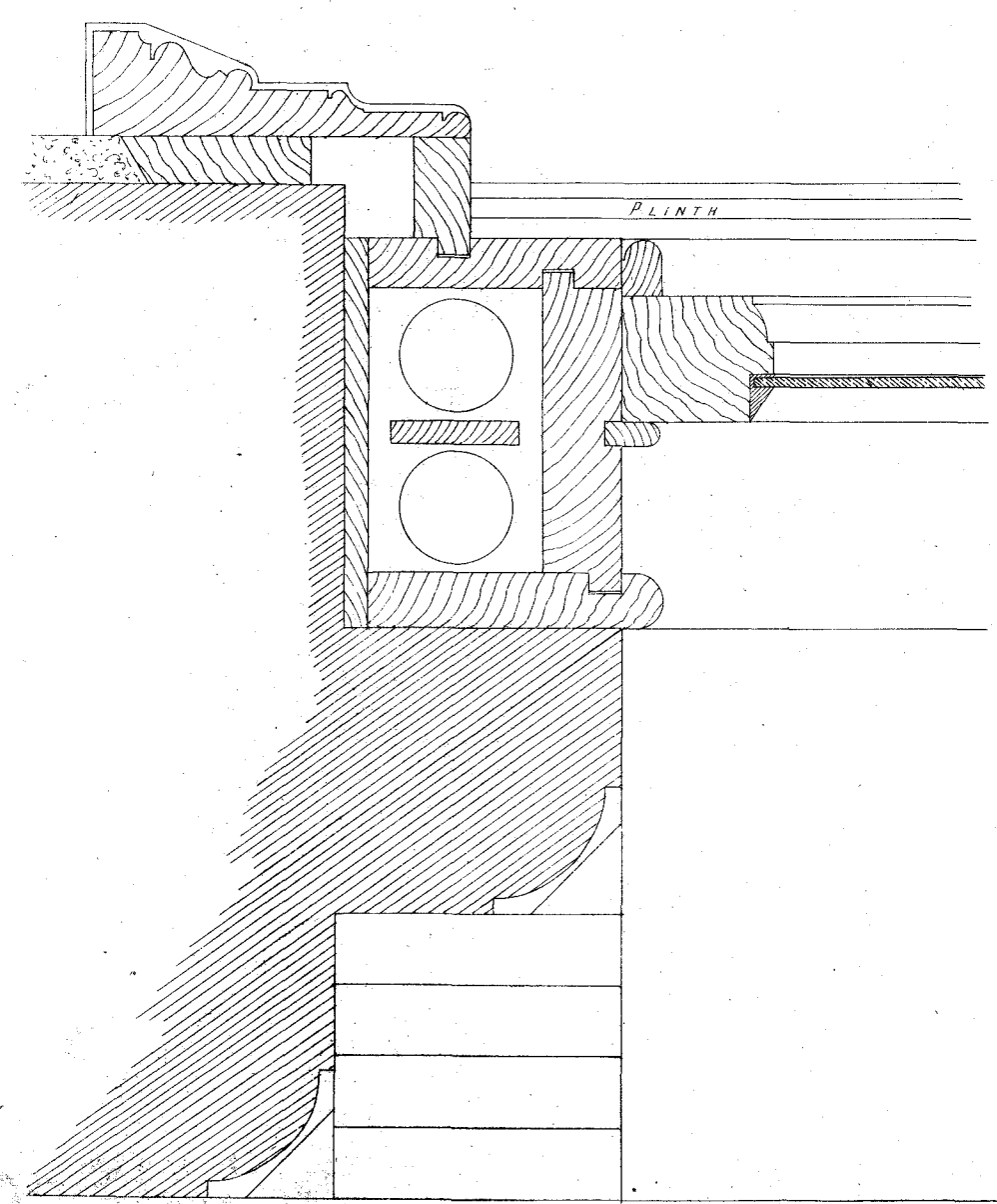
PLAN OF WINDOW FRAME, SASH & C.
