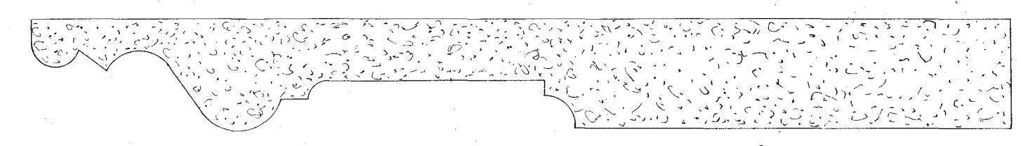
SECTION OF 12" CEMENT SKIRTING (Full size)
