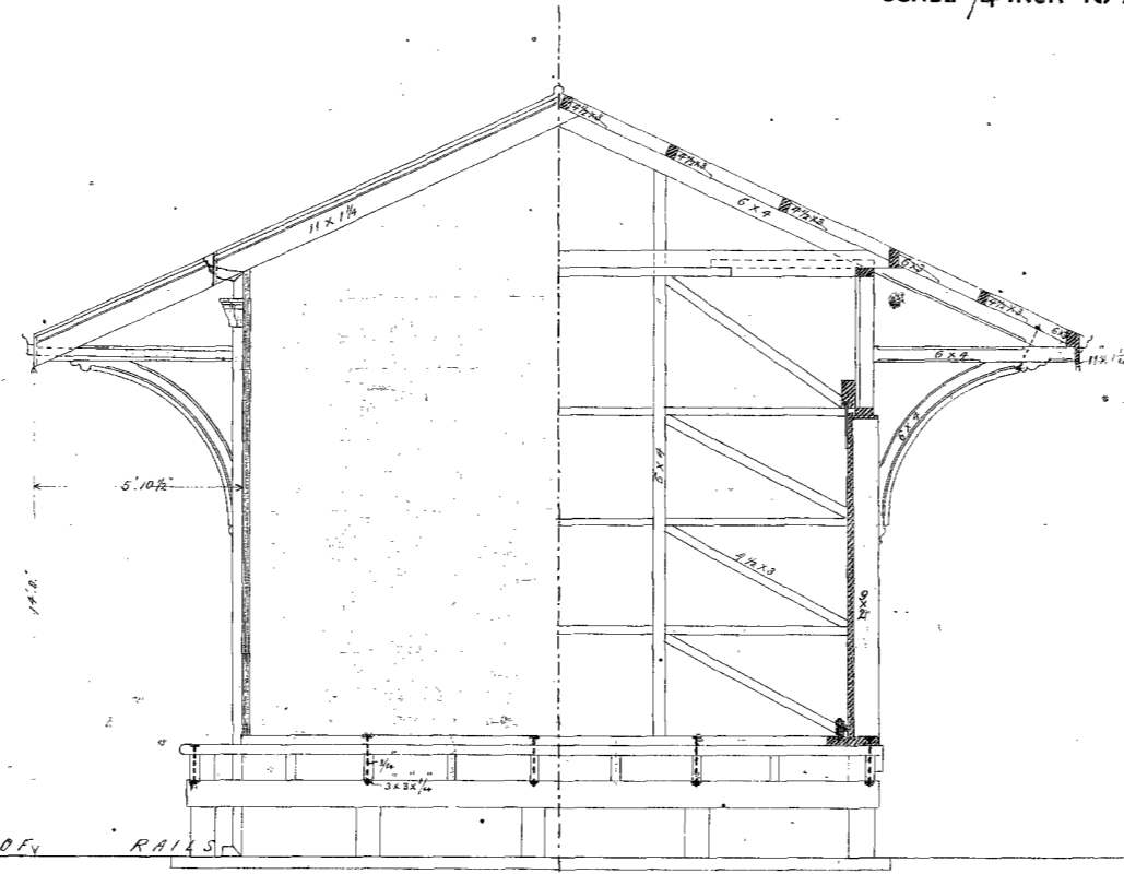
ELEVATION SECTION
