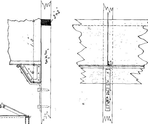
Detail of Bracket and part of Joist 1/4 IN. SCALE
