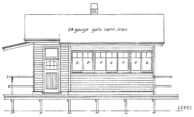
— ELEVATION TO PLATFORM —
