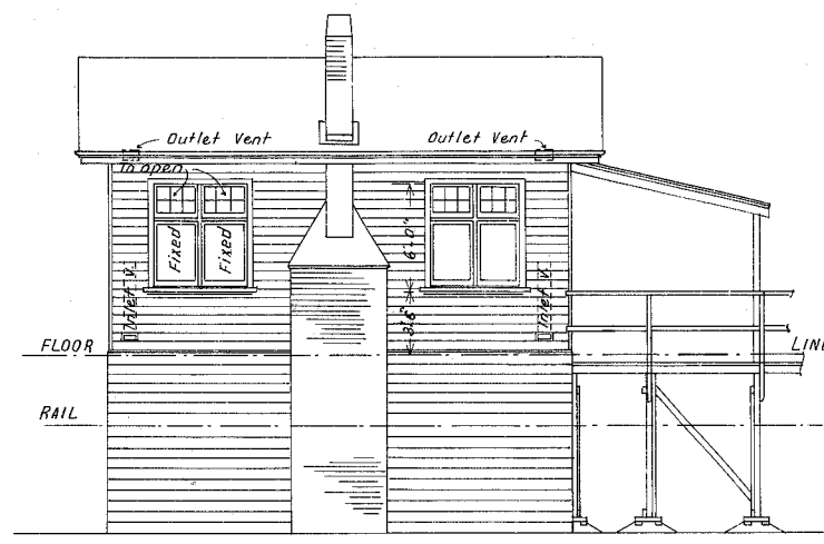
— ELEVATION TO APPROACH —
