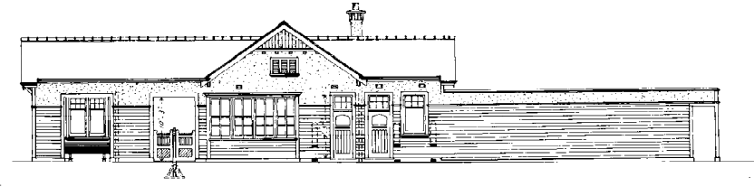
ELEVATION TO PLATFORM (UP SIDE)
