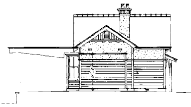
END ELEVATION (UP SIDE)
