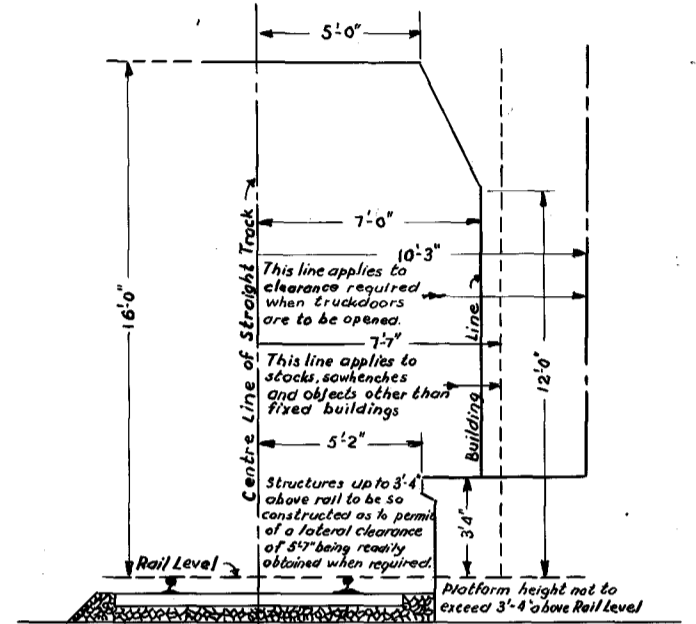
DIAGRAM SHOWING CLEARANCES TO BE OBSERVED ON PRIVATE SIDINGS WHERE TRACK IS STRAIGHT Where structures are to be built adjacent to curved tracks, turnouts and the approaches thereto, additional lateral clearance above that shown on this diagram is essential. The additional amount required is obtainable on application.
