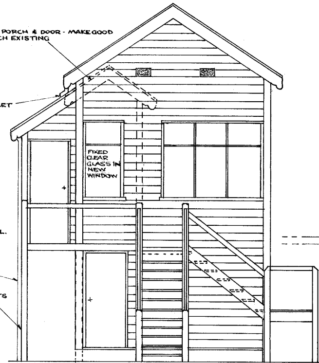
EAST ELEVATION SCALE \frac{1}{4}'' = 1'-0''
