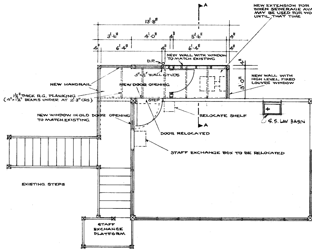
PLAN SCALE \frac{1}{4}'' = 1'-0''
