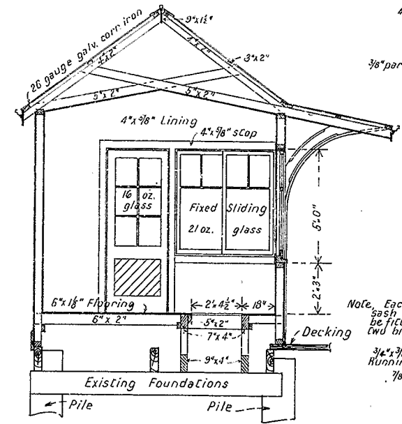
— CROSS SECTION —
