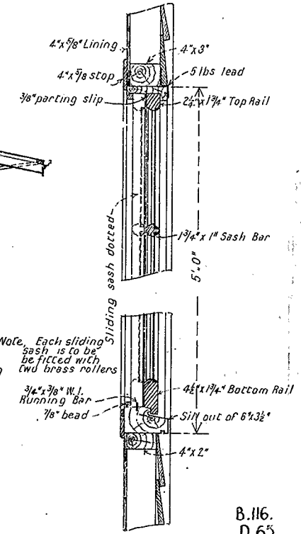
— SECTION THROUGH — — FIXED SASH — — 1" = 1 FOOT —
