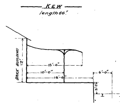
Cross Section of Verandahs Scale - 10 FT to 1"
