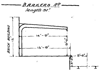
Cross Section of Verandahs Scale - 10 FT to 1"
